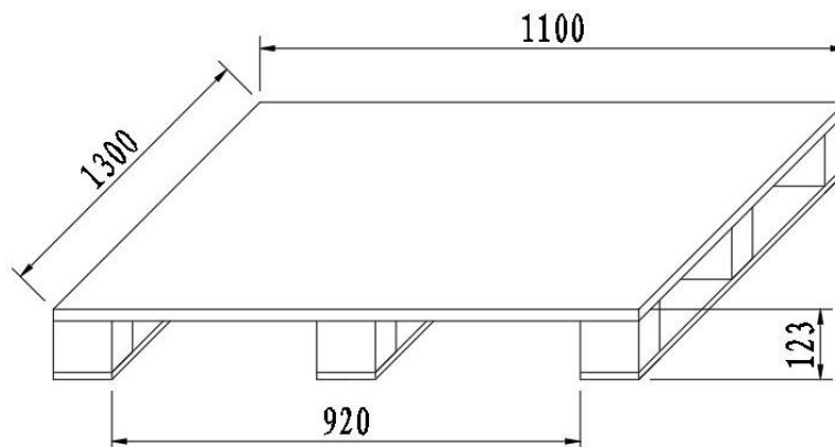
Figure 1 Schematic diagram of the card board
