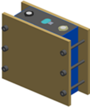
Side view of cell shaft 电池上夹具图
